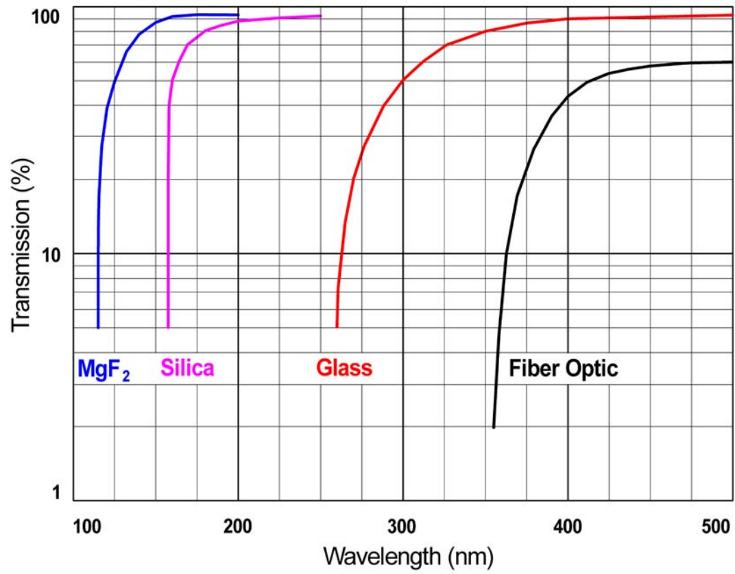
Typical Transmission of Input Window Materials
